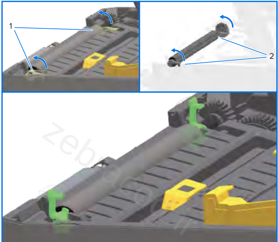
1 Platen bearings
