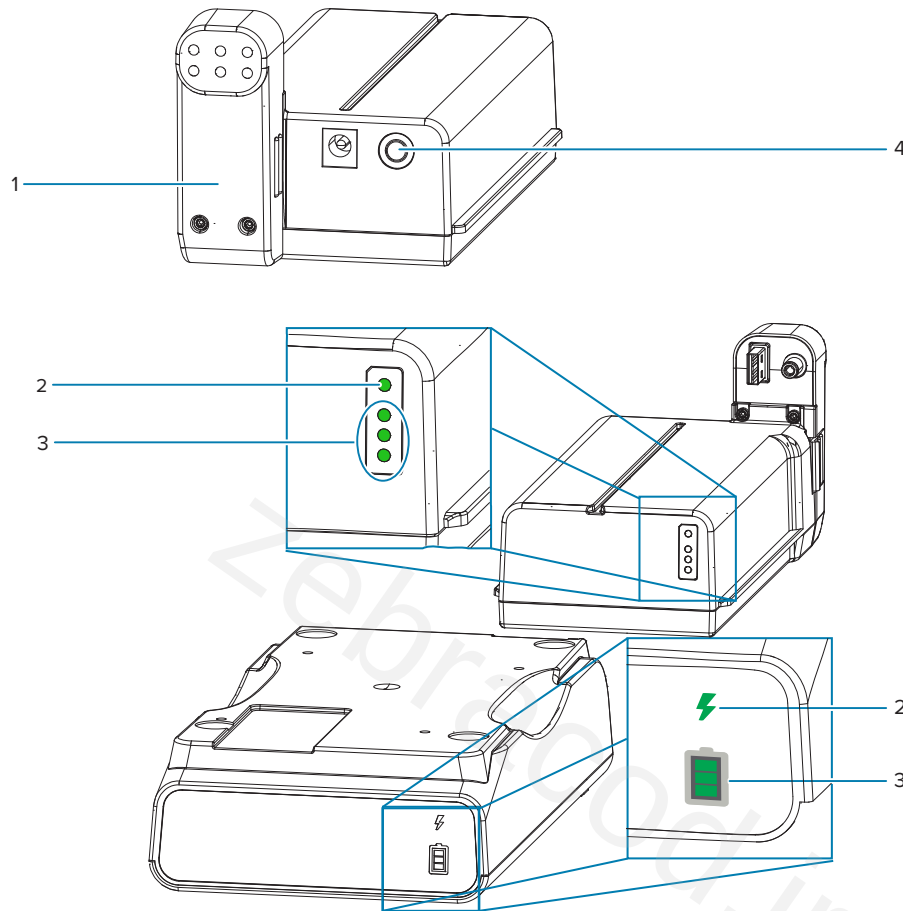
Figure 9 Battery Controls
