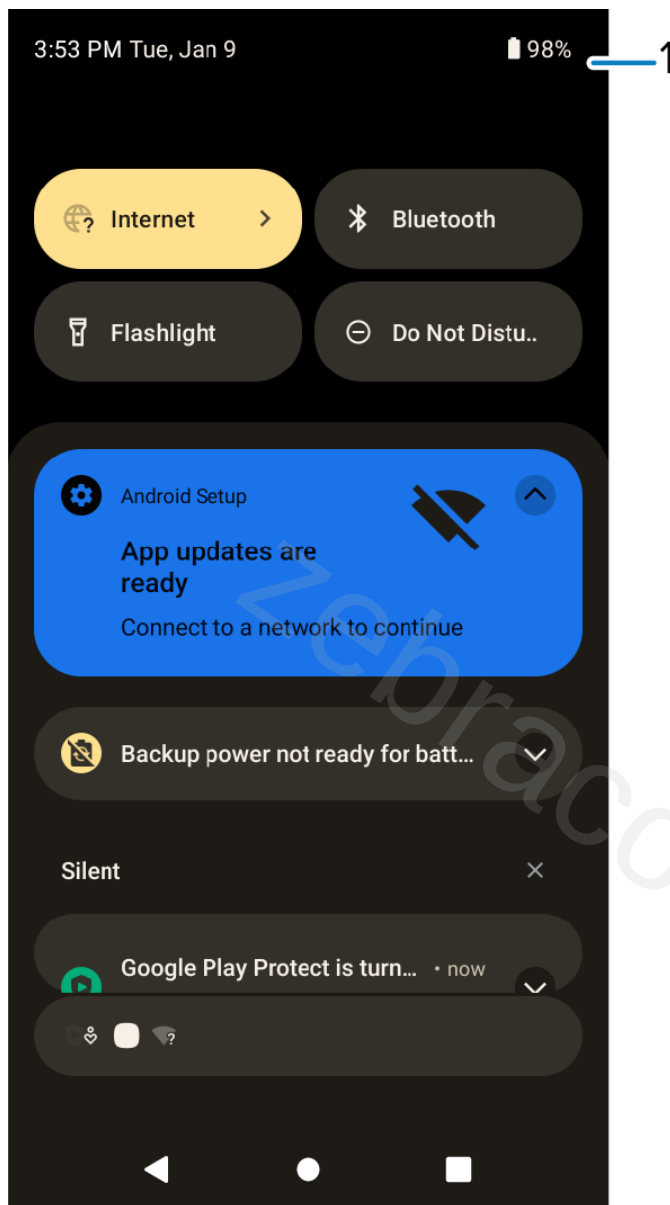
Figure 7 Android 13 Notification Panel
