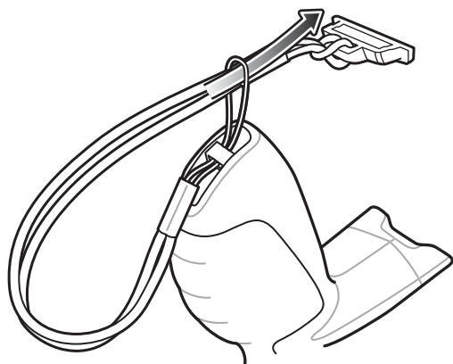
Figure 6-31 Tether Installation
