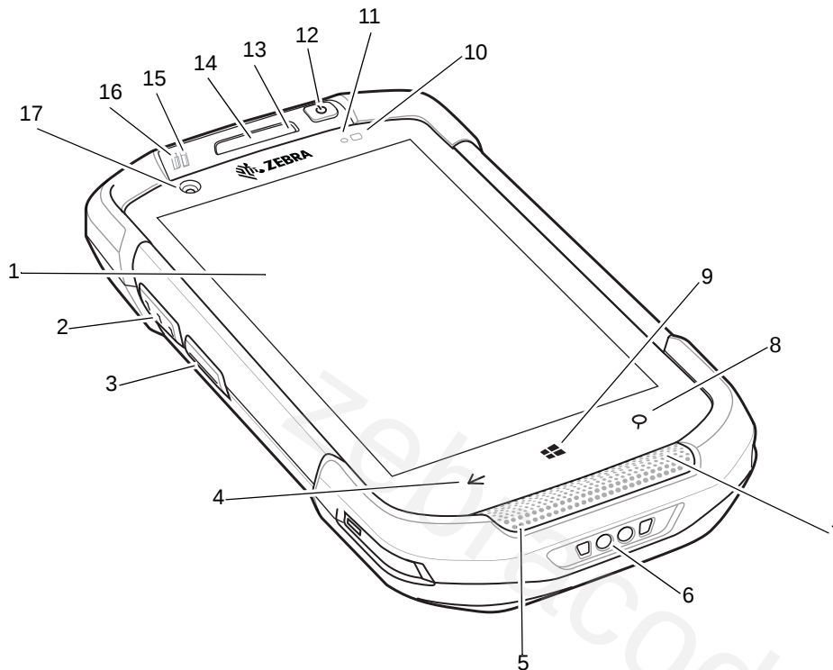
Figure 1-1 TC70x Front View
