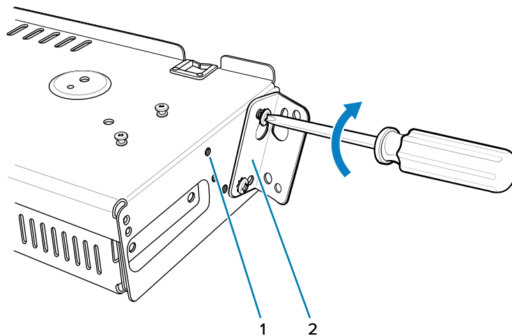
Figure 42 Flange 25° Position (4-Slot Battery Chargers)
