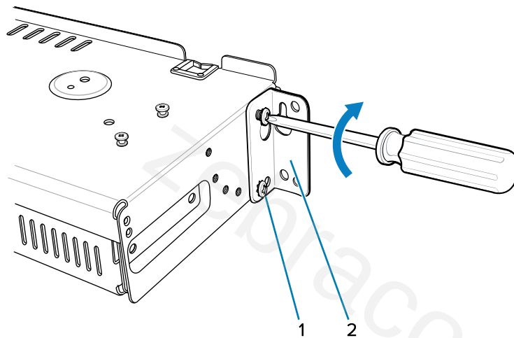
Figure 41 Flange Horizontal Position (5-Slot Cradles)
