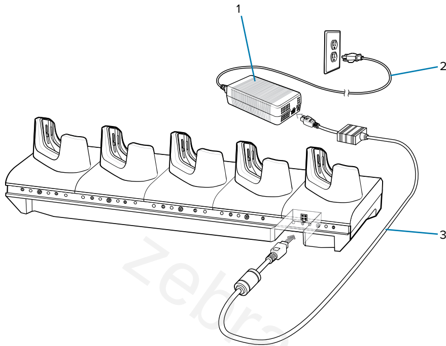
Figure 48 5-Slot Charge Only Cradle Setup
