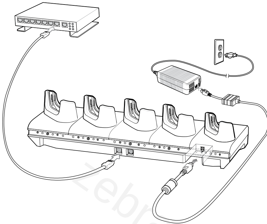
Figure 51 5-Slot Ethernet Cradle Setup
