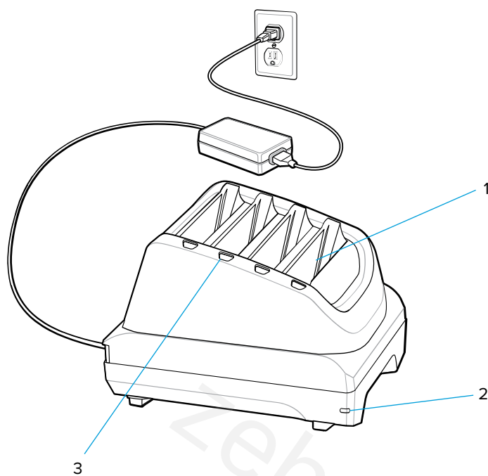
Figure 53 4-Slot Battery Charger
