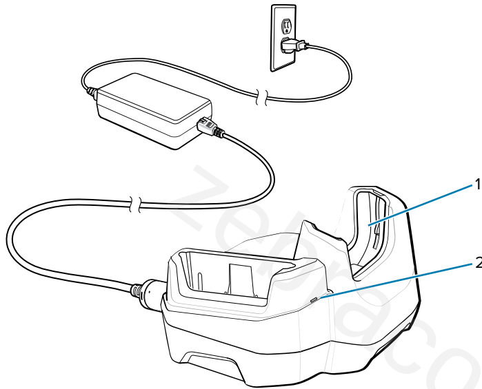
Figure 44 2-Slot USB/Ethernet Cradle
