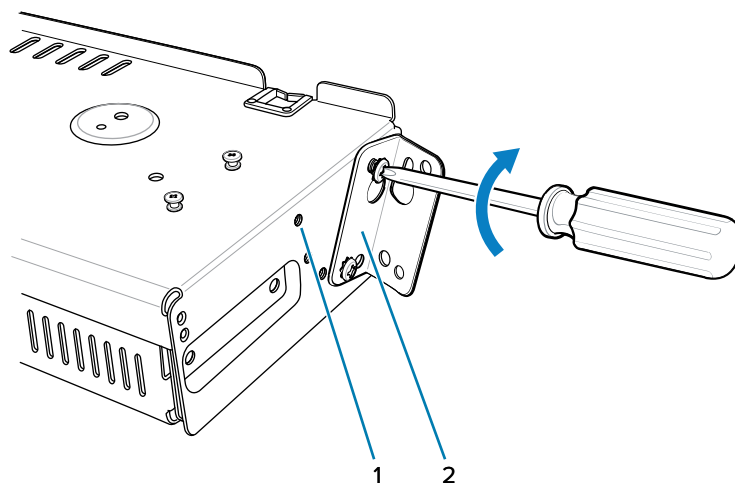
Figure 56 Flange 25° Position (4-Slot Battery Chargers)
