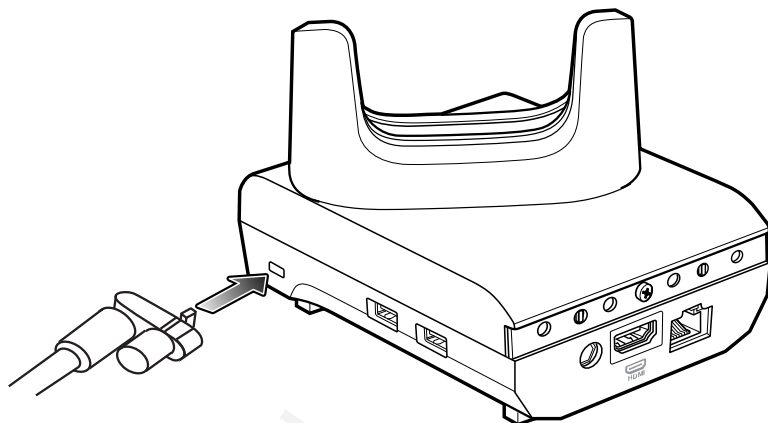
Figure 42 Securing Cradle with Kensington Lock
