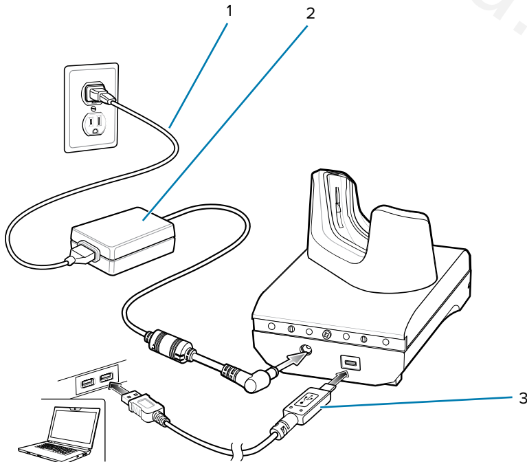
Figure 39 1-Slot USB Charge Cradle Setup
