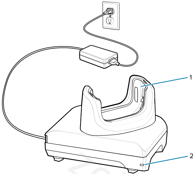
Figure 38 1-Slot USB Charge Cradle
