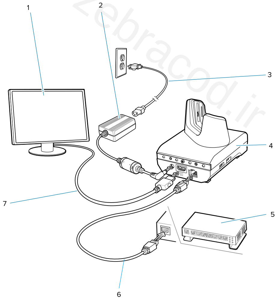
Figure 41 Workstation Cradle Setup
