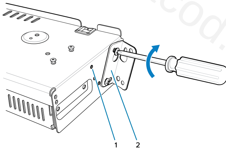
Figure 33 Flange 25° Position (4-Slot Battery Chargers)
