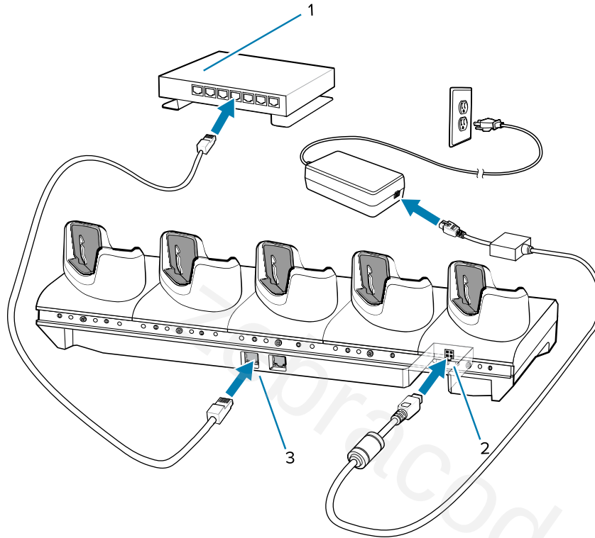
Figure 28 5-Slot Ethernet Cradle
