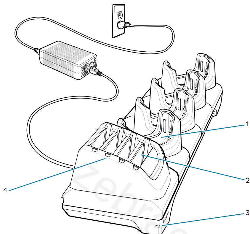
Figure 43 4-Slot Charge Only Cradle with Battery Charger
