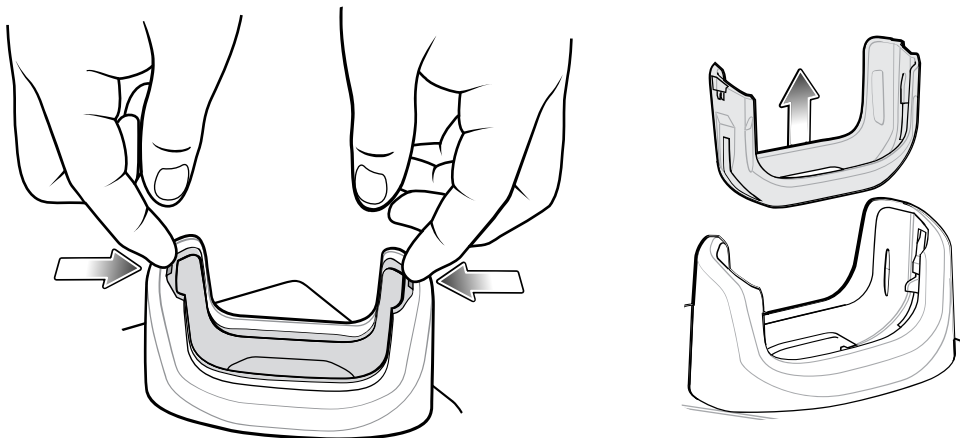
Figure 44 Remove the Insert from the Cup
