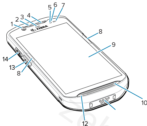
Figure 1 Front View
