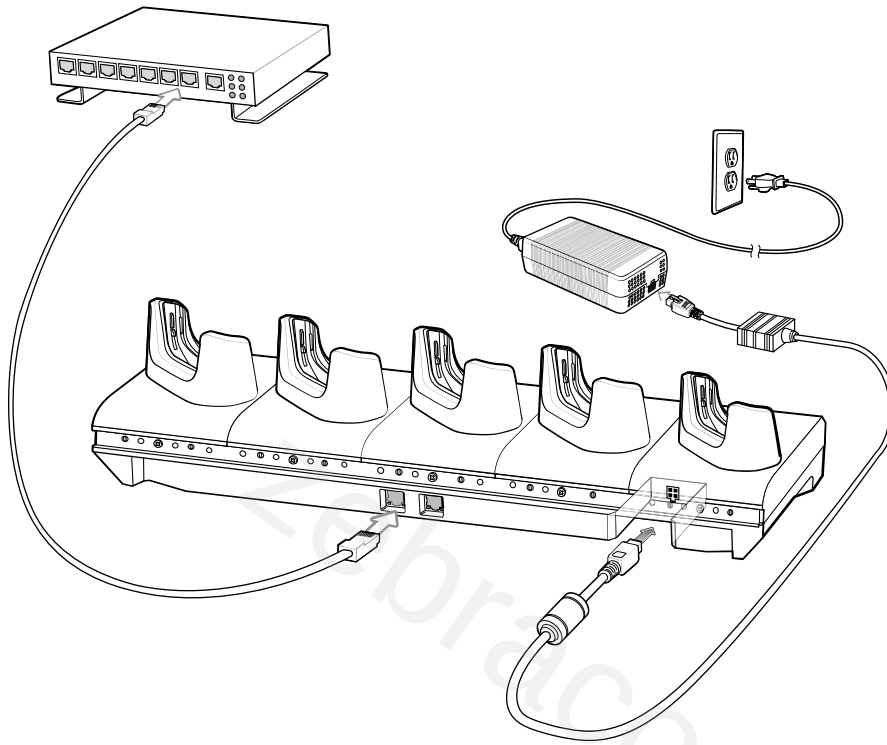
Figure 49 5-Slot Ethernet Cradle Setup
