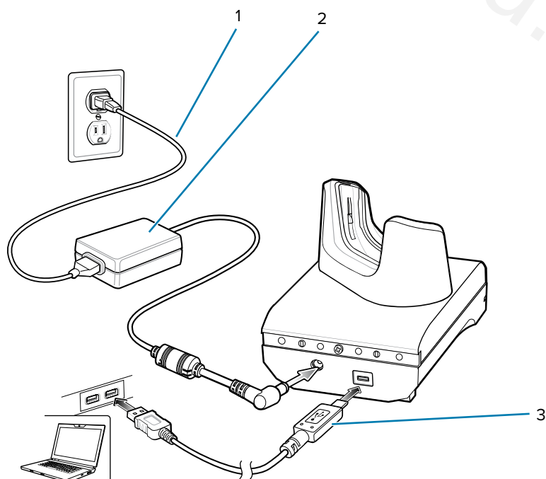
Figure 33 1-Slot USB Charge Cradle Setup
