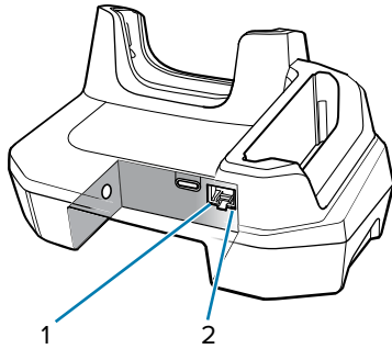
Figure 41 Ethernet LED Indicators
