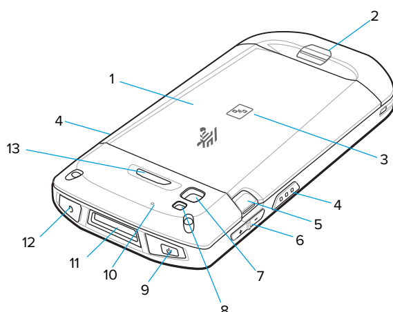
Figure 2 Rear View
