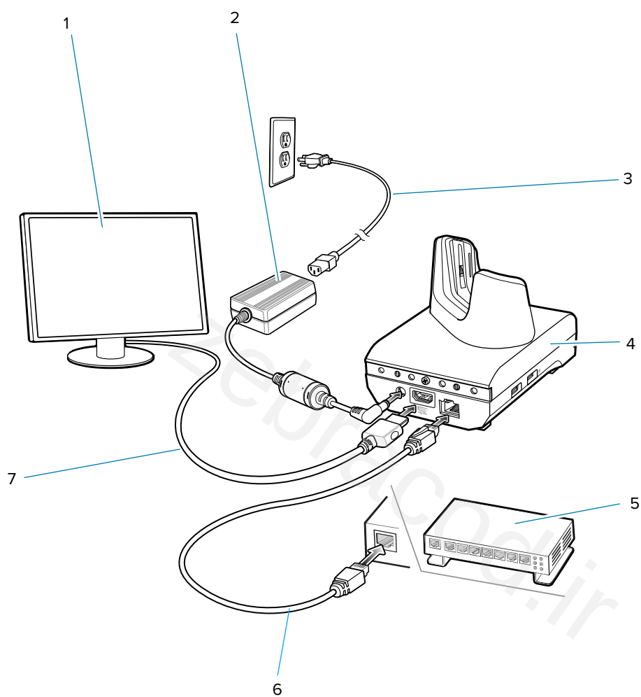
Figure 35 Workstation Cradle Setup
