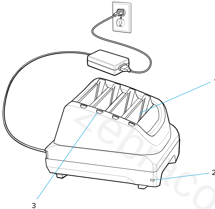
Figure 51 4-Slot Battery Charger
