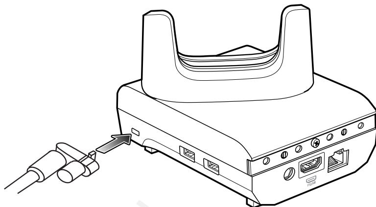
Figure 36 Securing Cradle with Kensington Lock
