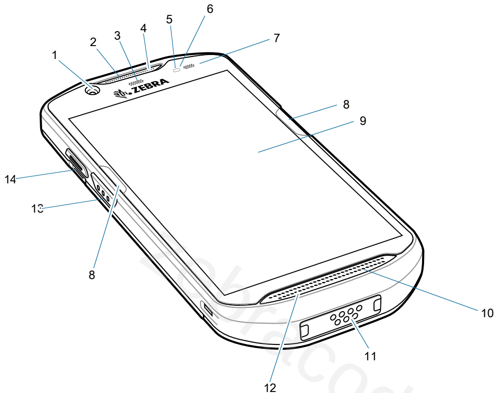
Figure 1 Front View
