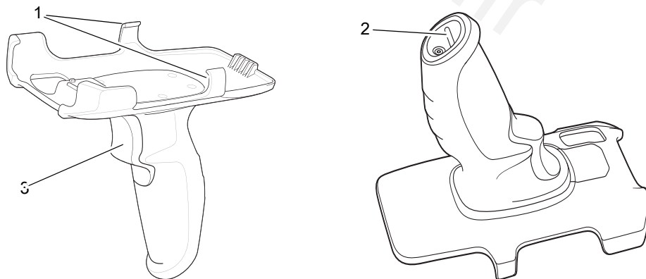
Figure 28 Trigger Handle
