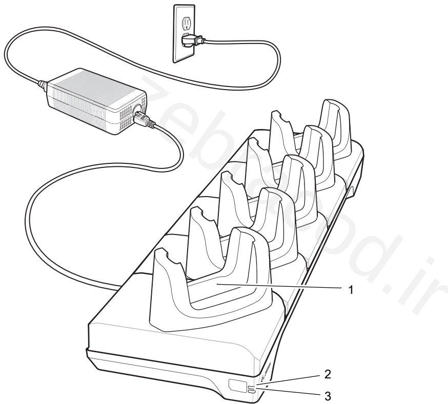
Figure 23 5-Slot Ethernet Cradle
