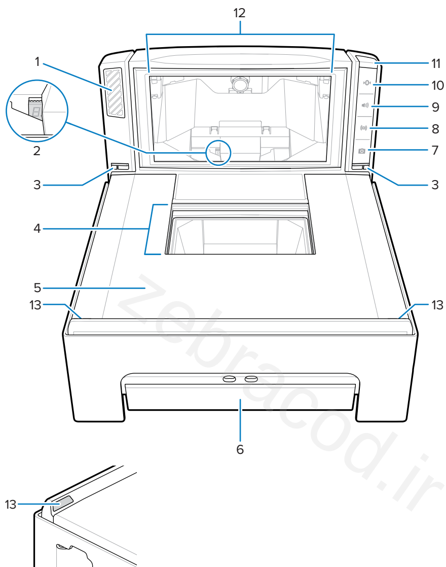
Figure 1 Front View
