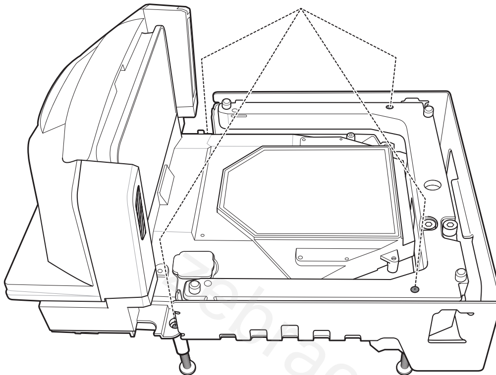
Figure 1-5 Leveling Screws
