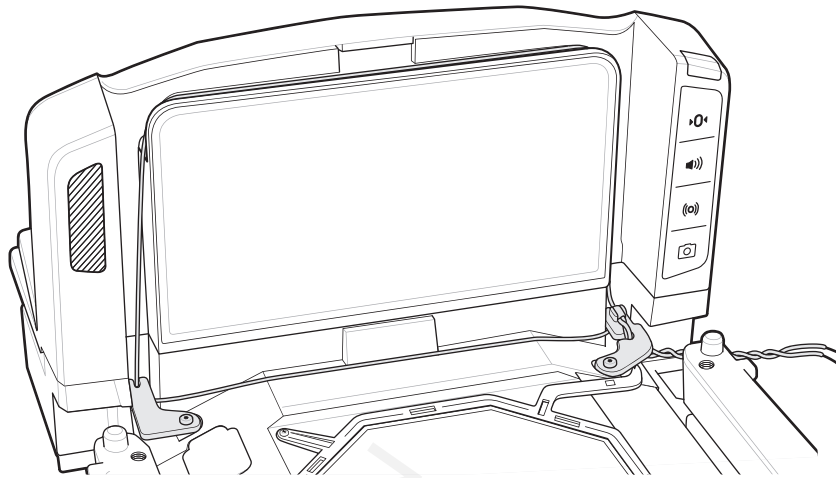
Figure 3-37 Completed Installation
