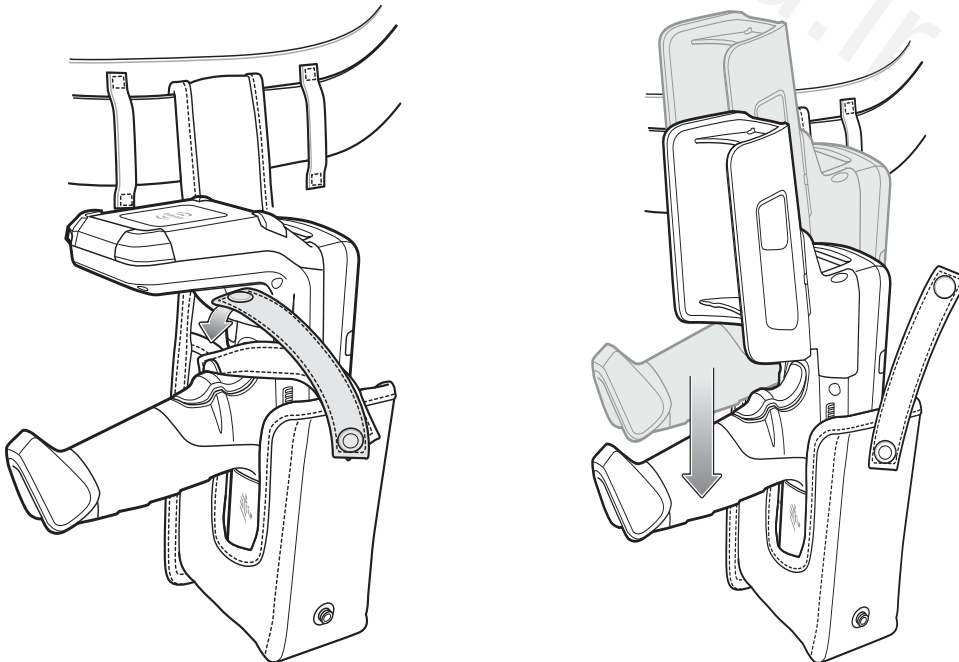
Figure 34 Insert MC3300xR
