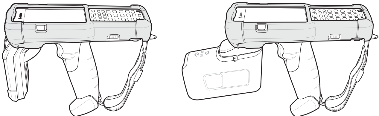
Figure 30 Place Rubber Boot Over Top of MC3300xR
