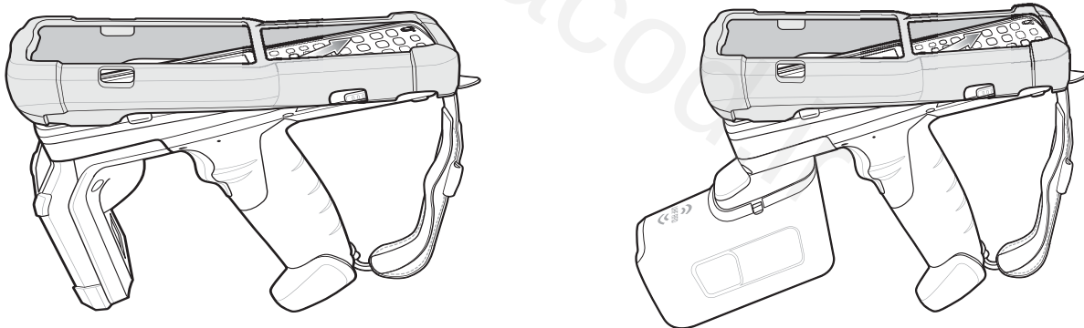
Figure 29 Slide MC3300xR into Bottom of Rubber Boot
