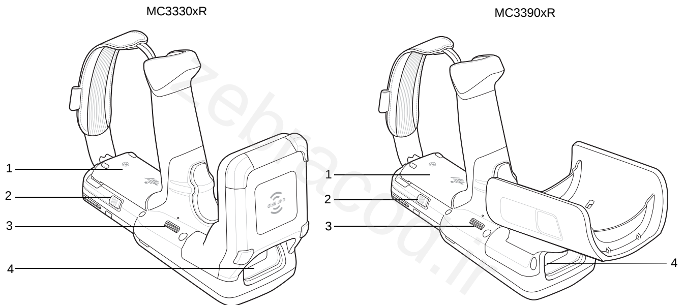
Figure 4 Parts on the Device - Bottom Views
