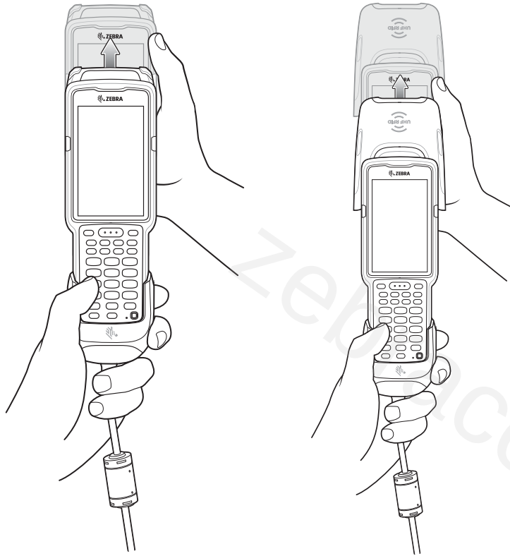
Figure 24 Disconnecting the USB Charge Cable
