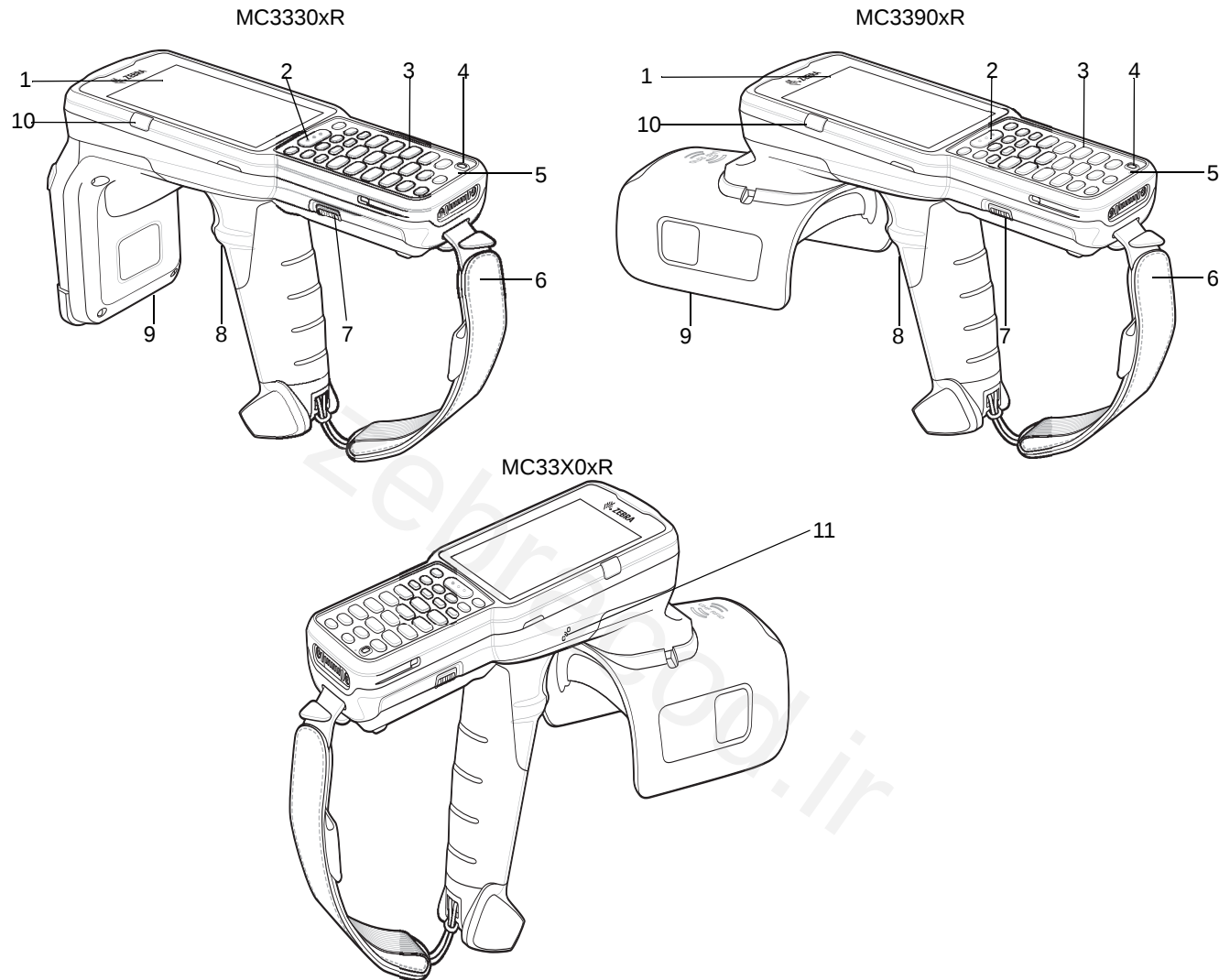
Figure 3 Parts on the Device - Side Views
