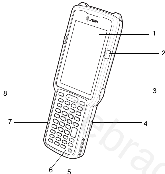
Figure 6 MC3300x-S Front View
