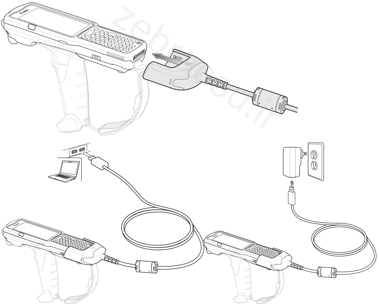
Figure 33 USB Charge Cable
