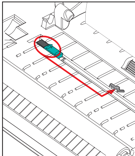
Off Center Blackline Sensing Only
