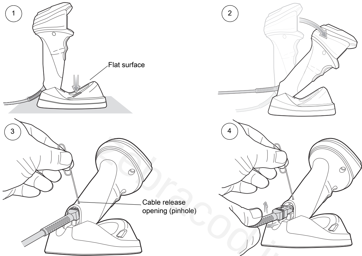
Figure 3 Removing the Cable
