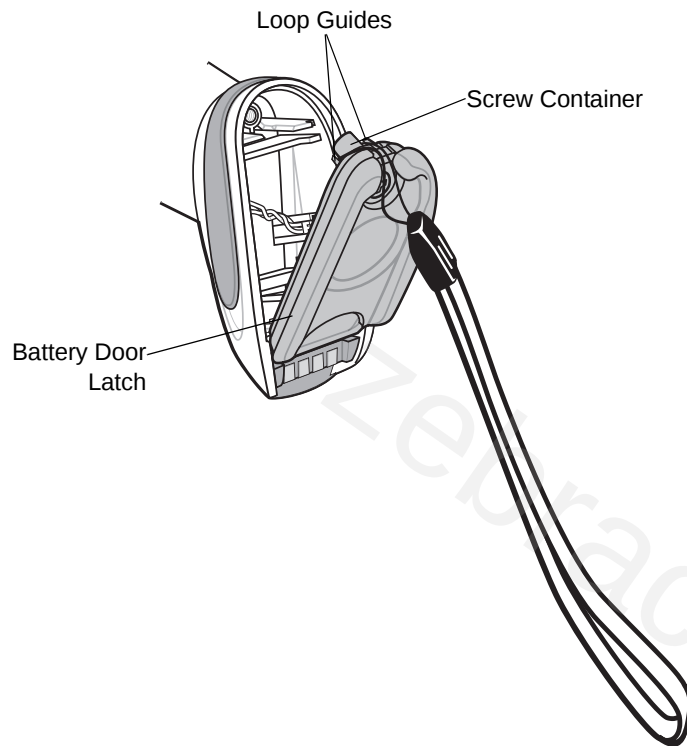
Figure 1-15 Attaching Lanyard
