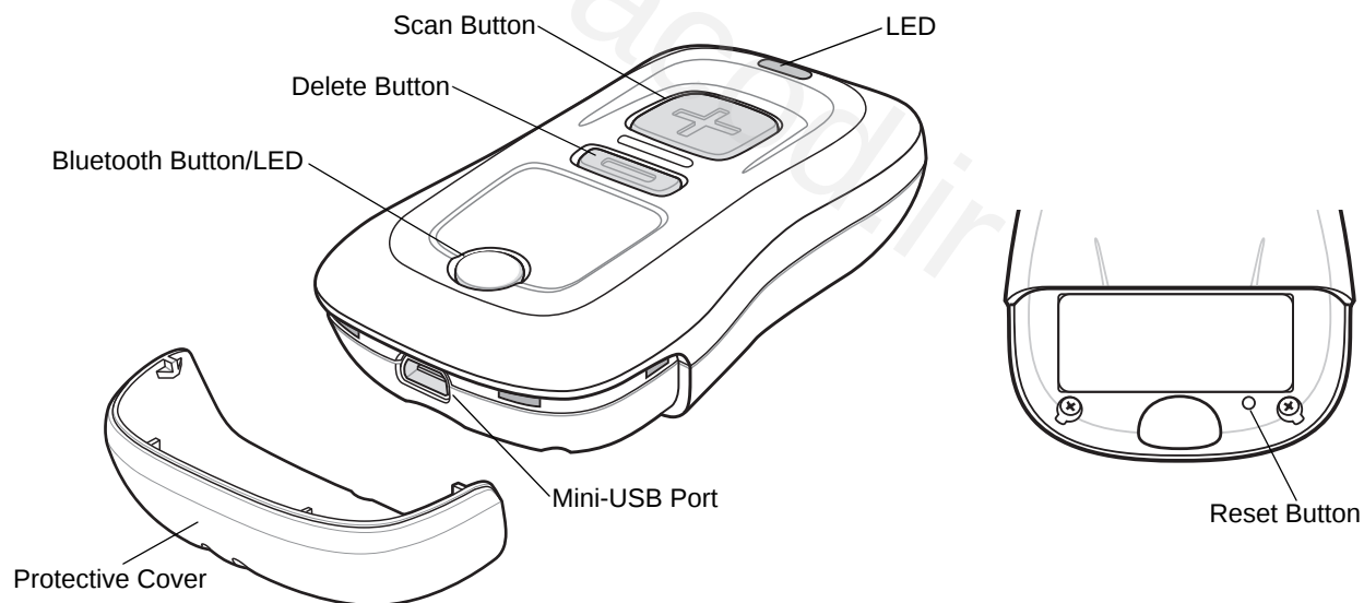
Figure 1-1 CS3000 Series Scanner
